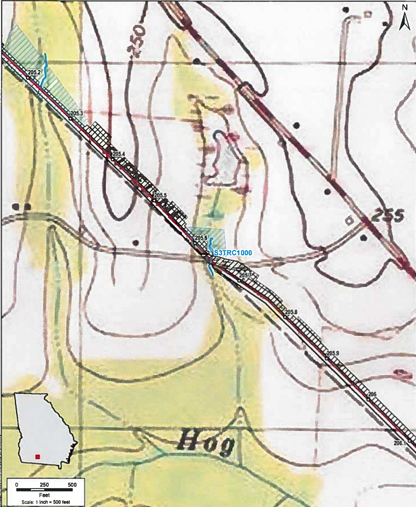
FIGURE 2 SABAL TRAIL PROJECT S3TRC1000 USGS OVERVIEW
