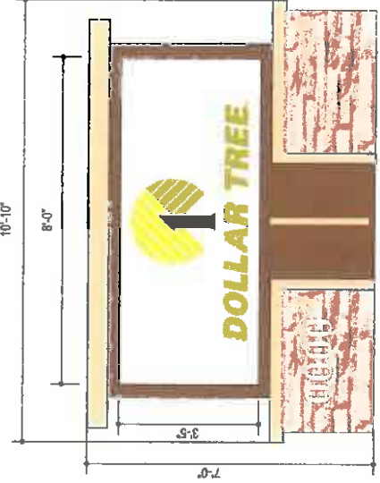
Main ID - 1 Single Tenant ID with Provision for 1 Lighted Tentant Panel
